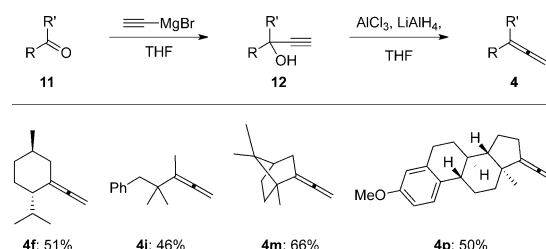
Scheme 7. Two-step synthesis of allenic substrates from ketones (see SI for details).
