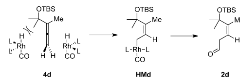
Scheme 5. Proposed reason for stereoinduction.
